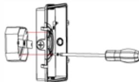
3. Fix the mounting box on the J-BOX
